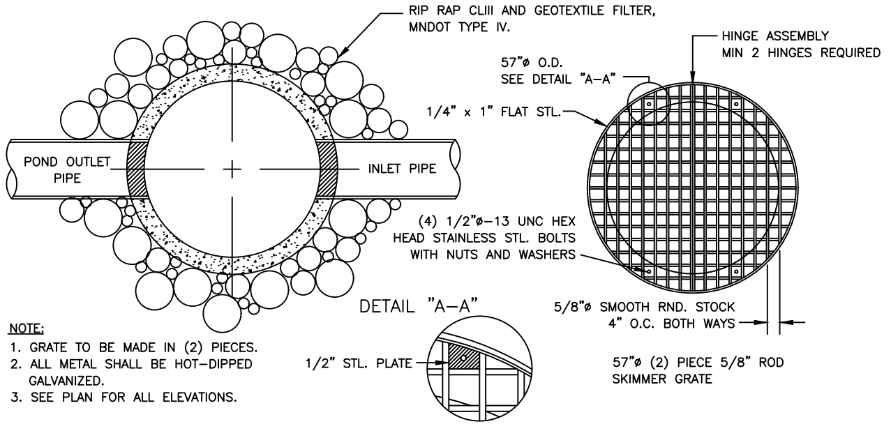
TOP VIEW
